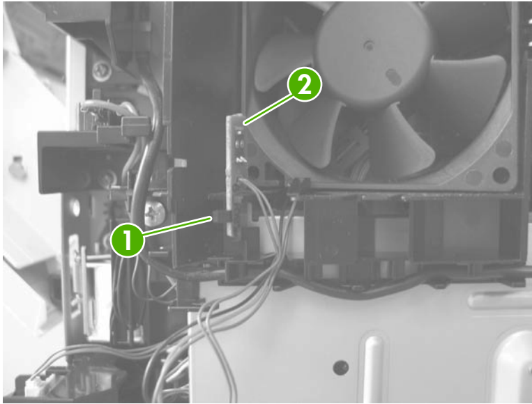
Figure 2-79 Remove the main fan, fan duct, and the environmental sensor PCA (2 of 3)
