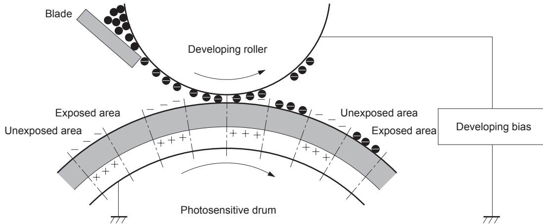
Figure 1-20 Print cartridge
