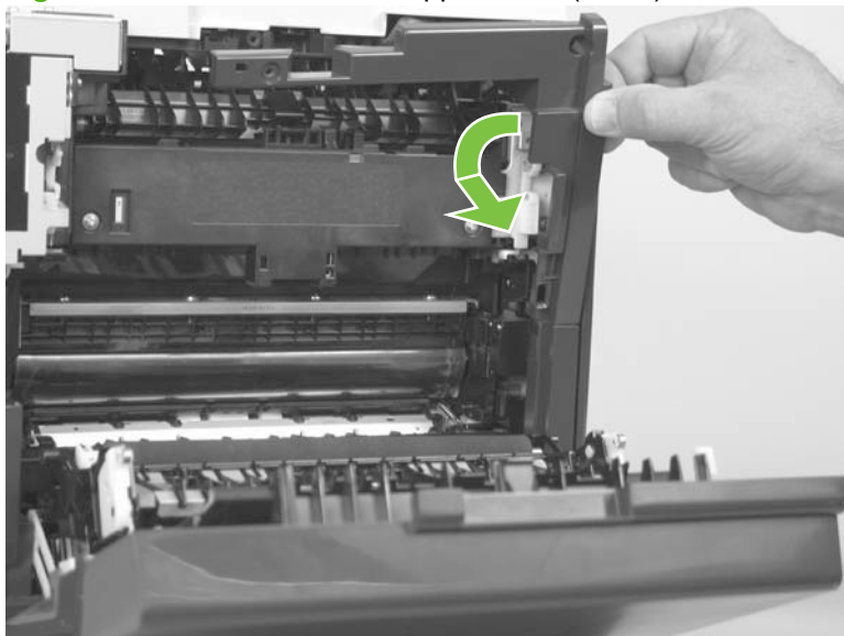
Figure 6-67 Remove the rear-upper cover (2 of 2)
