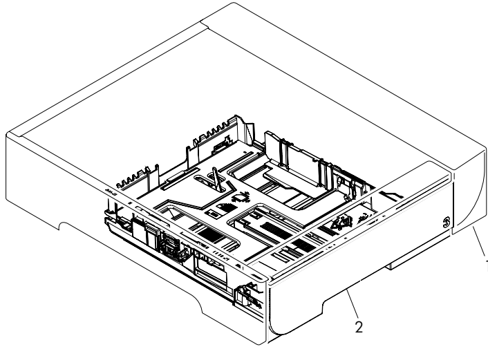
Figure 8-12 Optional 250-sheet paper cassette
