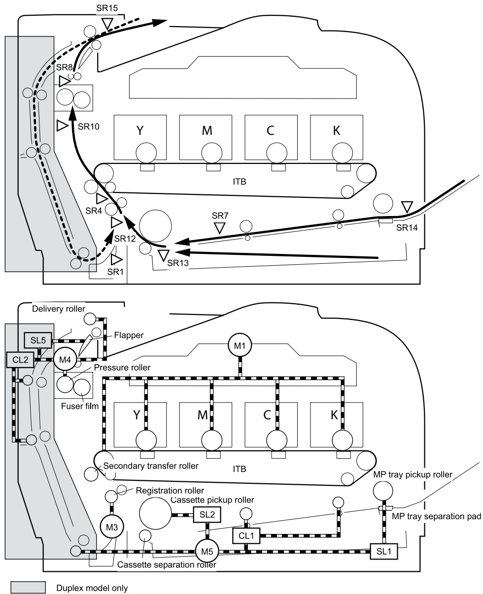
Figure 5-21 Pickup-and-feed system
