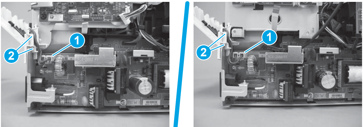
Figure 1-1890 Disconnect one connector
