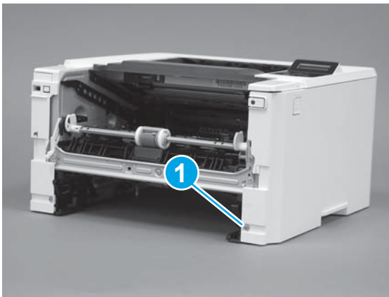
Figure 1-754 Remove one screw
