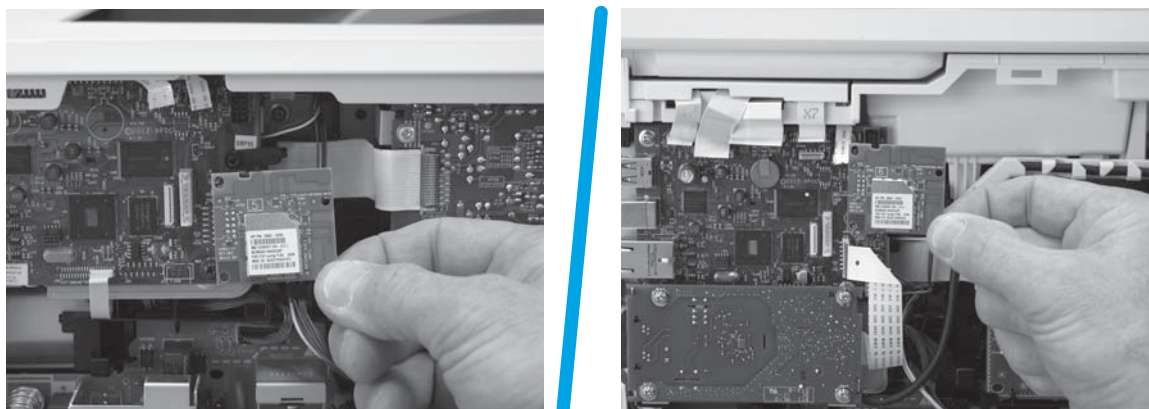
Figure 1-874 Install the PCA
