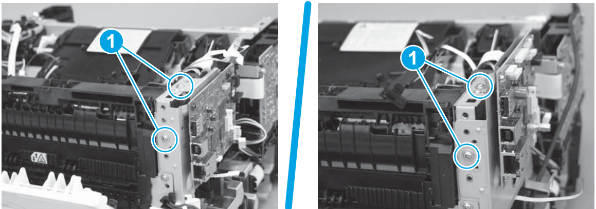
Figure 1-1889 Remove two screws
