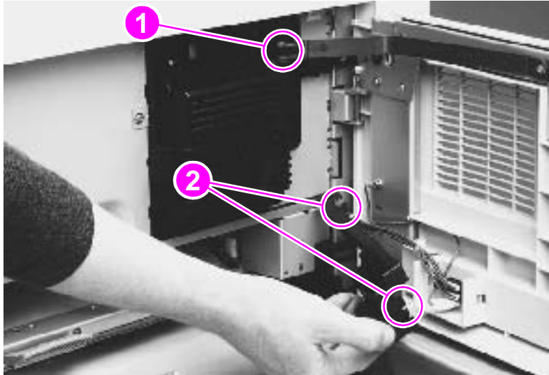
Figure 42. Right door (1 of 2)
