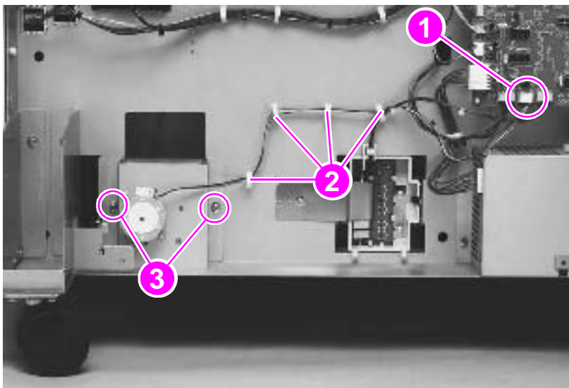
Figure 109. Drive assembly
