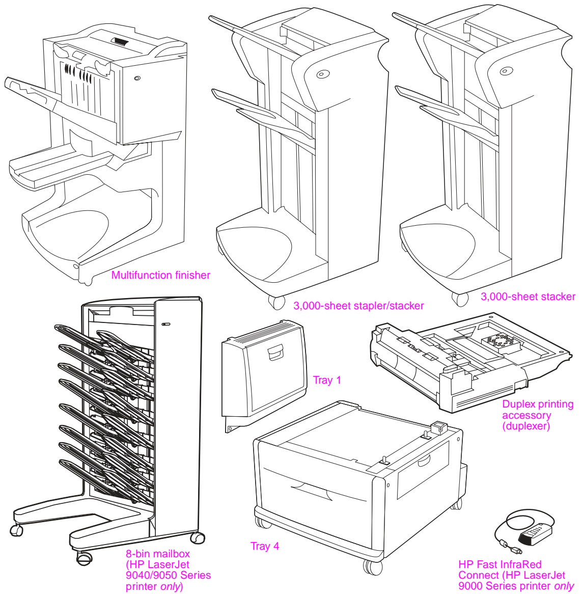
Figure 5. Optional accessories
