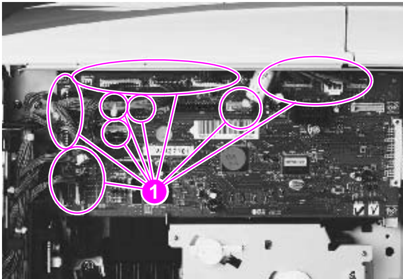
Figure 84. DC controller (1 of 2)
