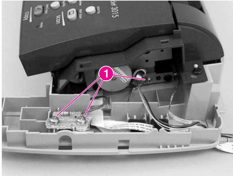
Figure 5-39. Remove the scanner assembly top cover (1 of 4)
