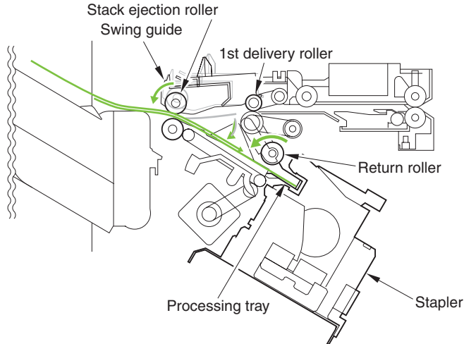
Figure 8-28 Paper path
