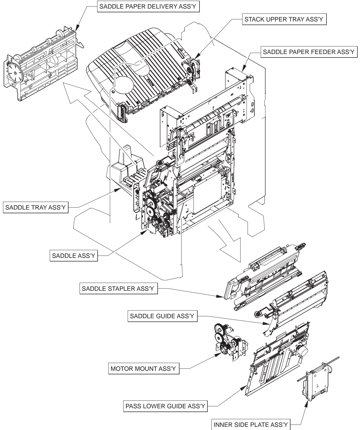
Figure 9-36 Booklet-maker unit
