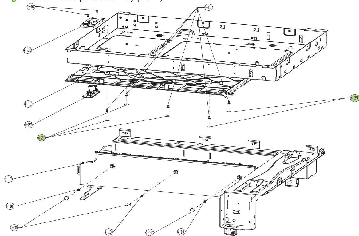
Figure 9-96 Plastic-parts assembly (2 of 2)
