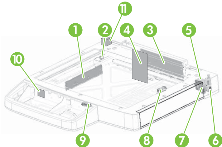
Figure 7-60 Components (scanner)
