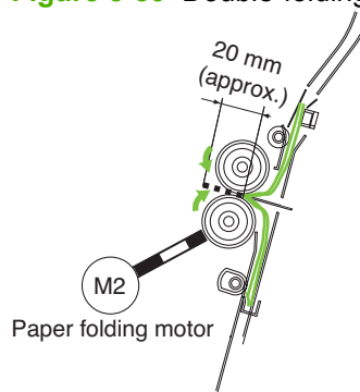
Figure 8-83 Double-folding process (3 of 5)
