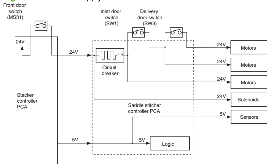
Figure 8-94 Power-supply route for the stacker unit
