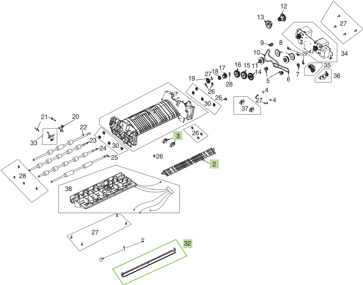
Figure 9-77 Backbone assembly
