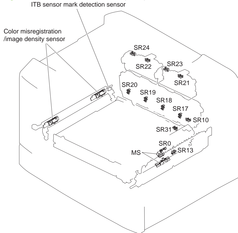
Figure 7-36 Product sensor locations (3 of 3)
