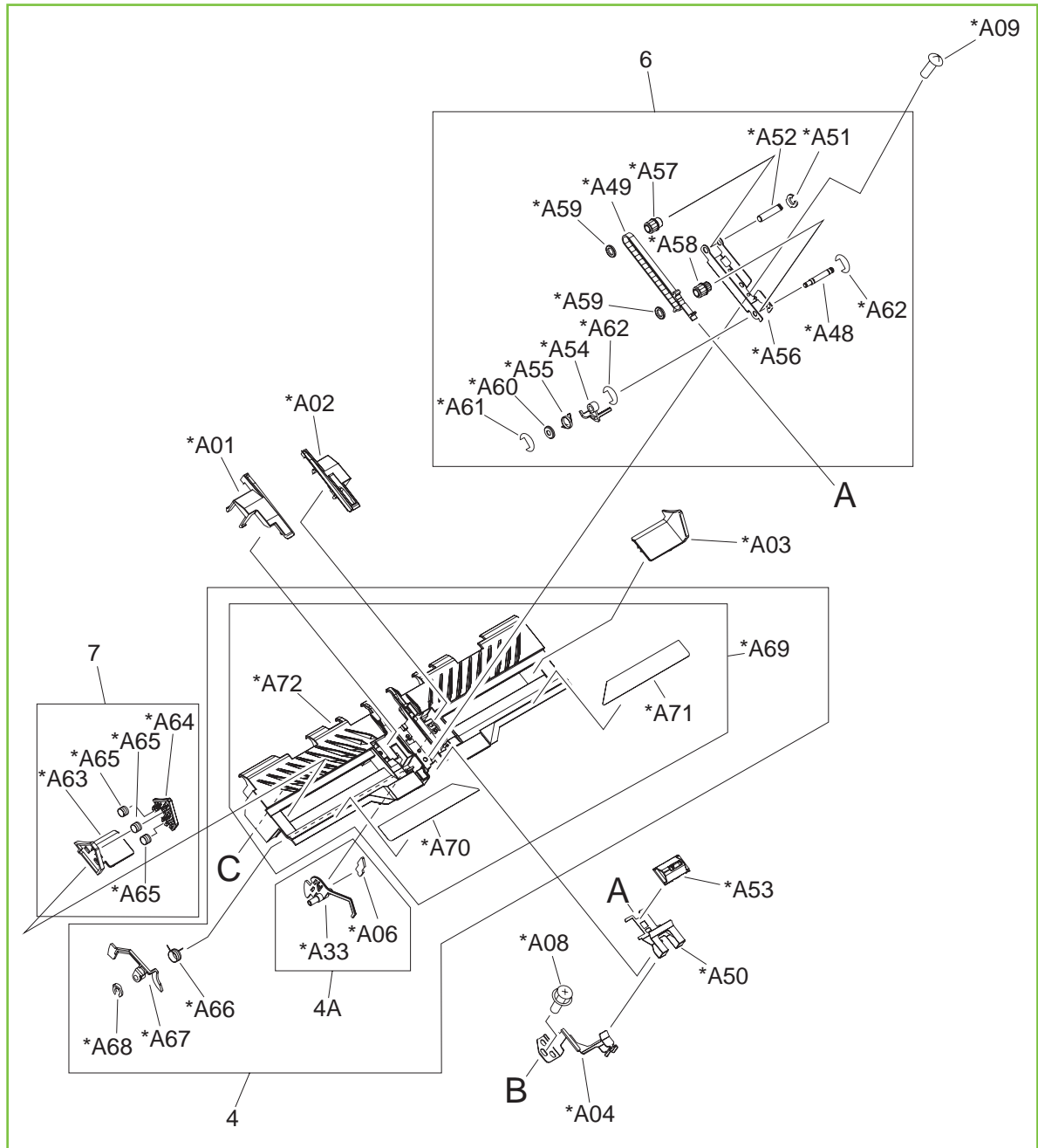
Figure 9-51 Operation-tray assembly (1 of 2) (stapler/stacker and booklet-maker)
