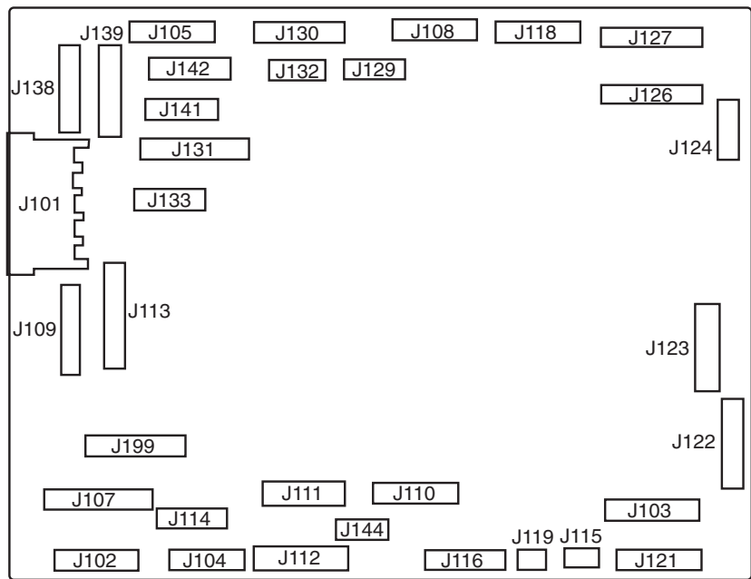
Figure 7-17 DC controller PCA
