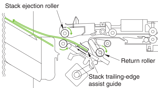
Figure 8-16 Paper path (5 of 5)
