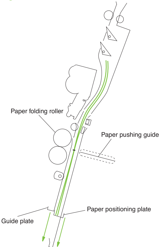
Figure 8-75 Stack sequence
