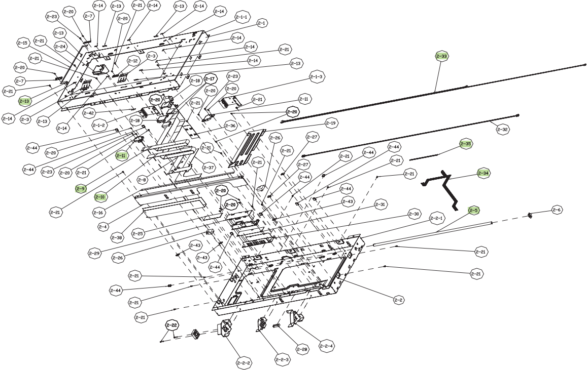
Figure 9-93 Main-frame assembly
