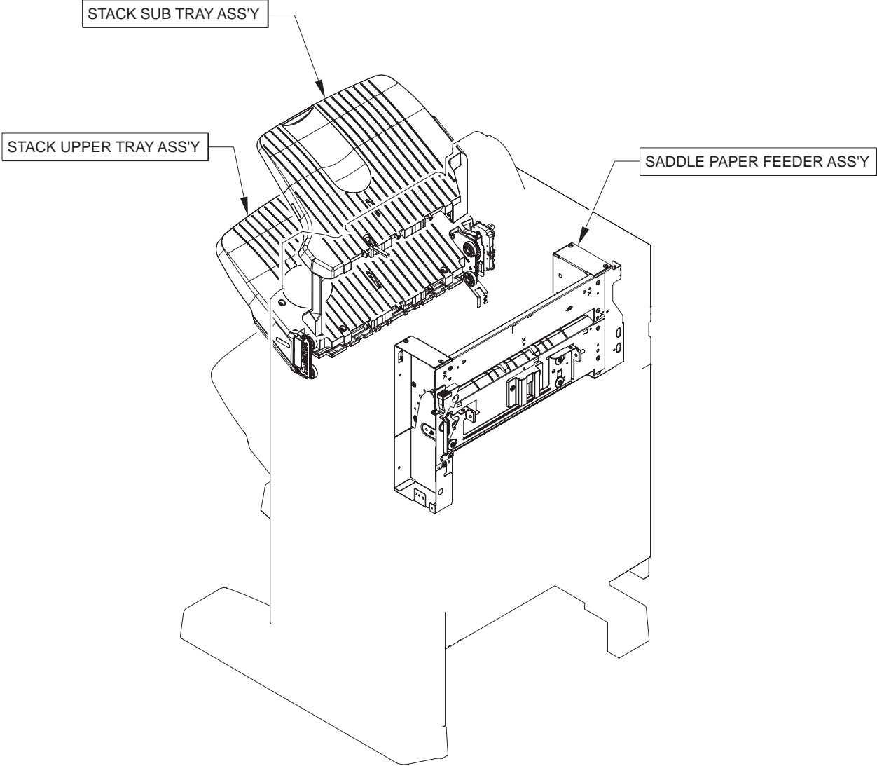
Figure 9-35 Stapler/stacker unit
