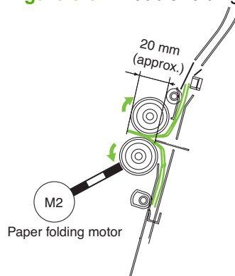
Figure 8-82 Double-folding process (2 of 5)
