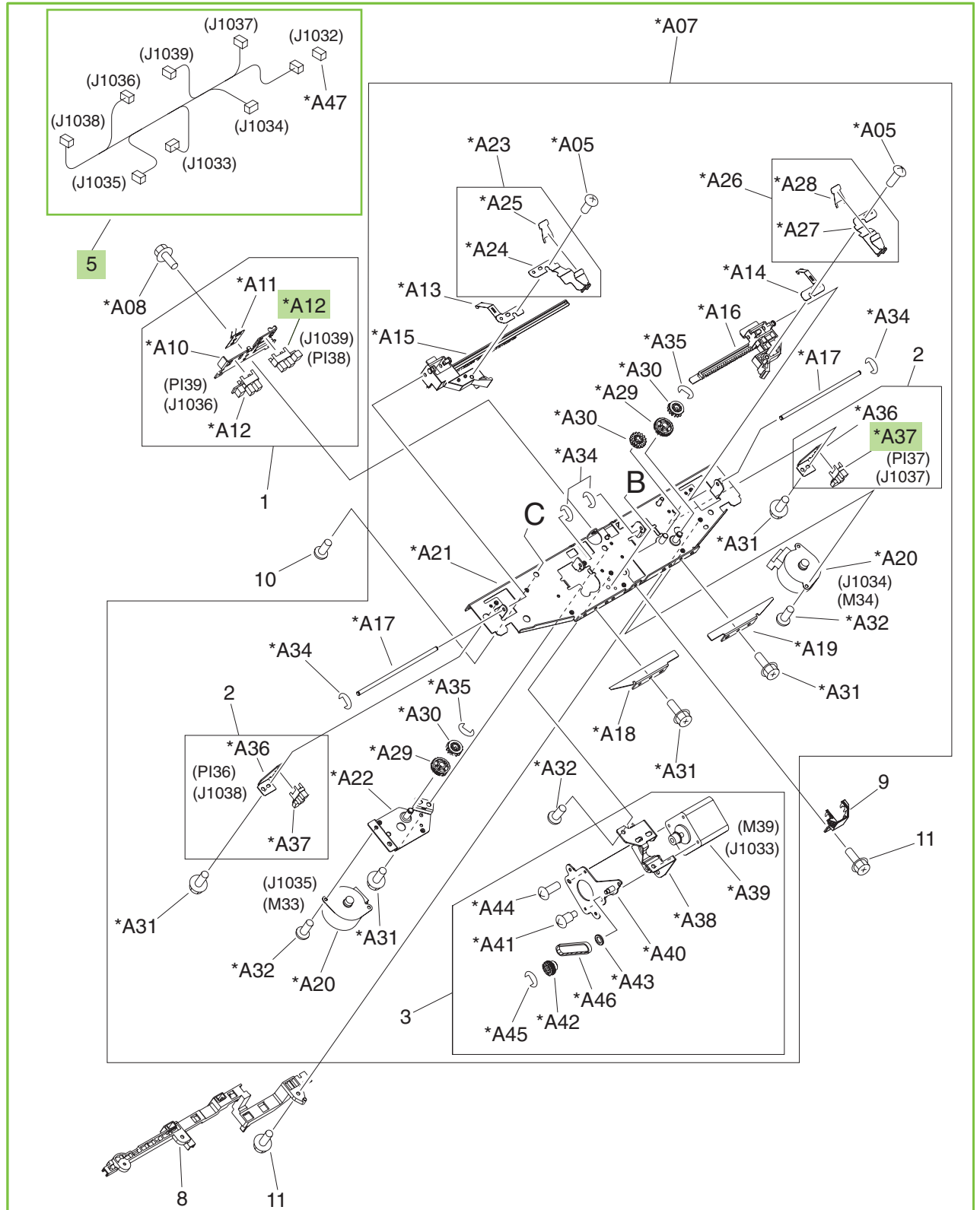
Figure 9-52 Operation-tray assembly (2 of 2) (stapler/stacker and booklet-maker)
