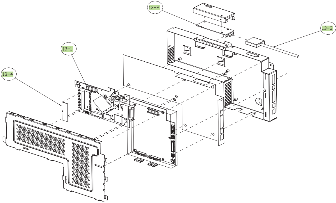
Figure 9-100 Havic assembly
