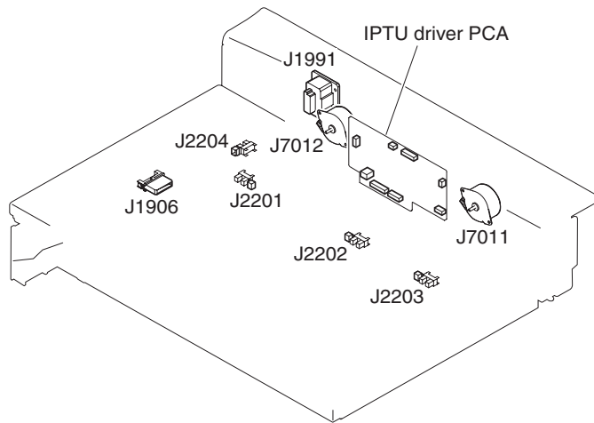
Figure 7-32 IPTU
