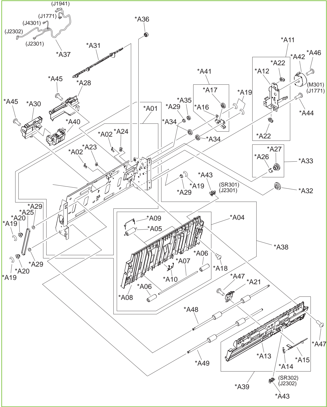
Figure 9-20 Printer duplexing-feed assembly
