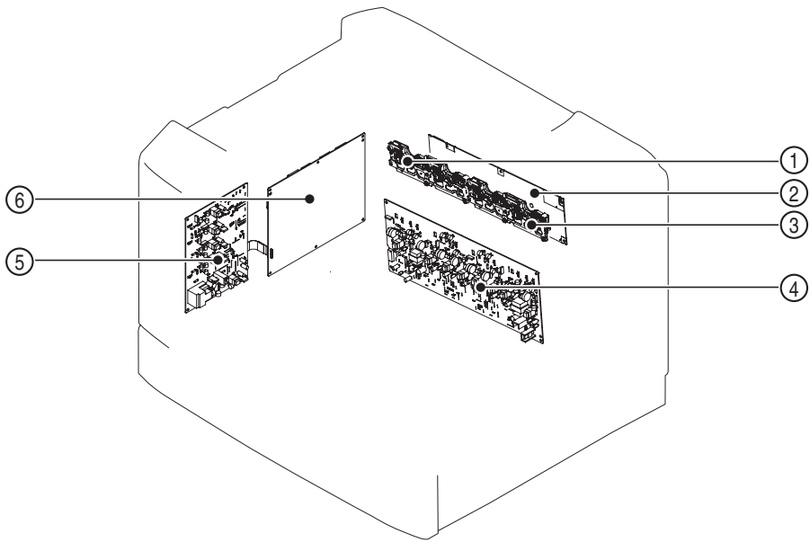
Figure 7-56 PCAs
