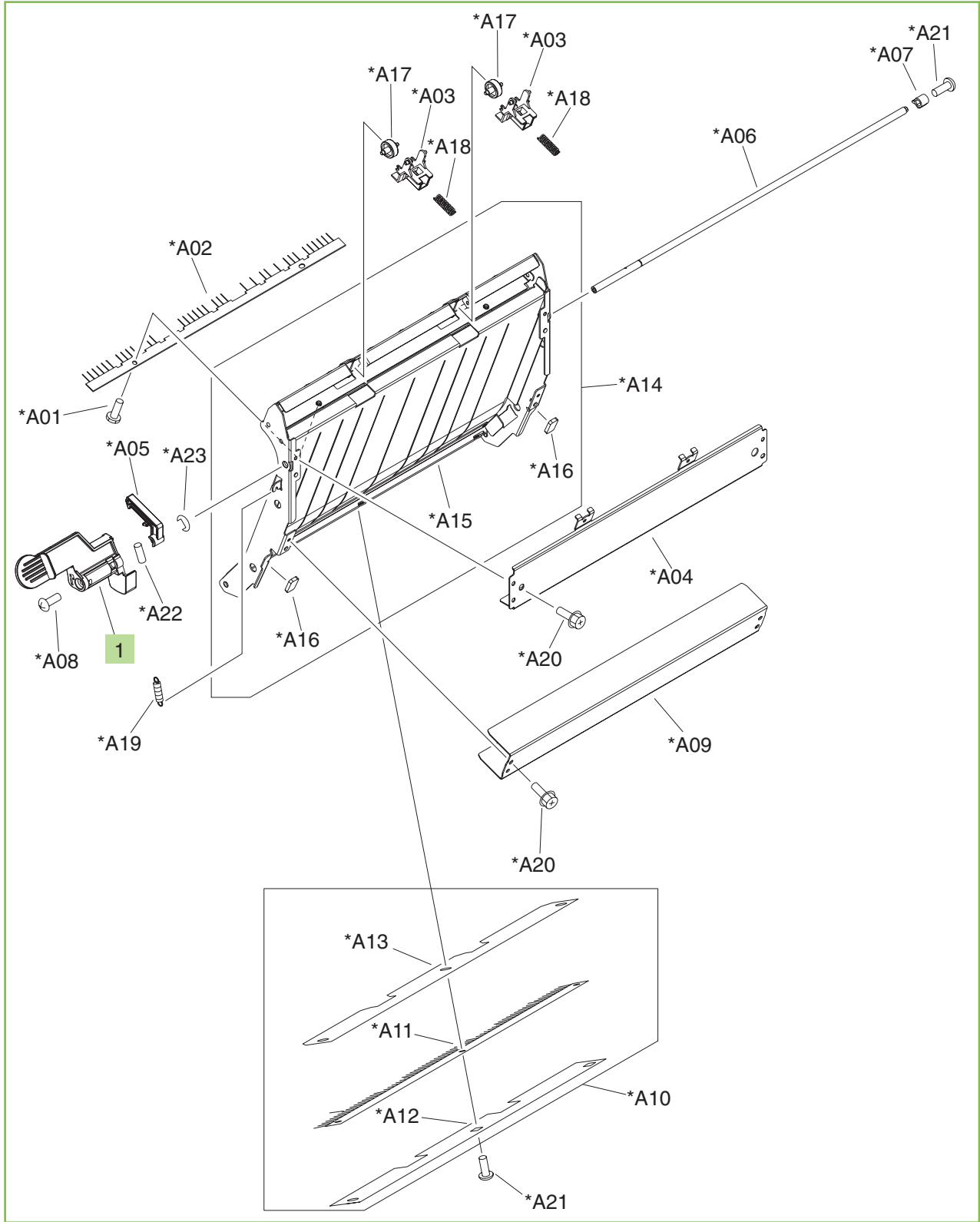
Figure 9-64 Saddle-guide assembly (booklet-maker)
