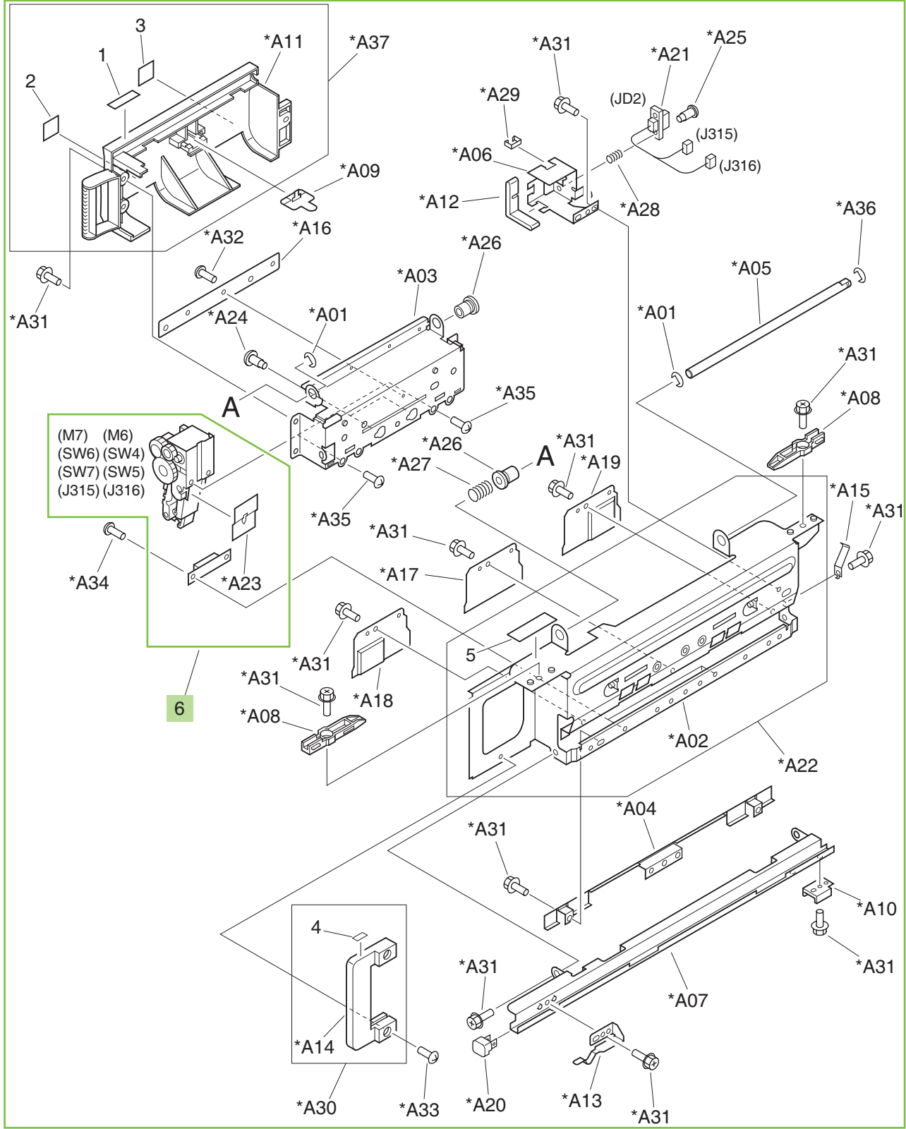
Figure 9-65 Saddle-stapler assembly (booklet-maker)
