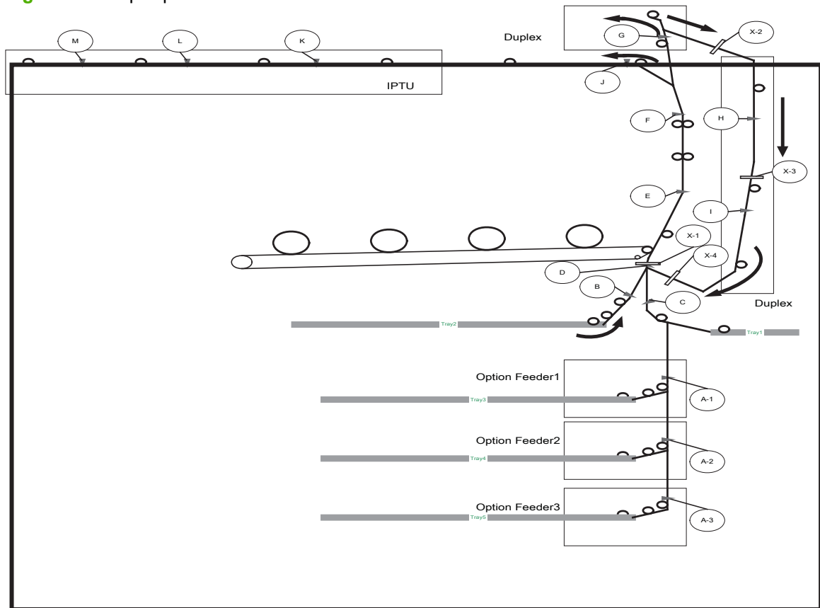
Figure 7-4 Paper-path sensors
