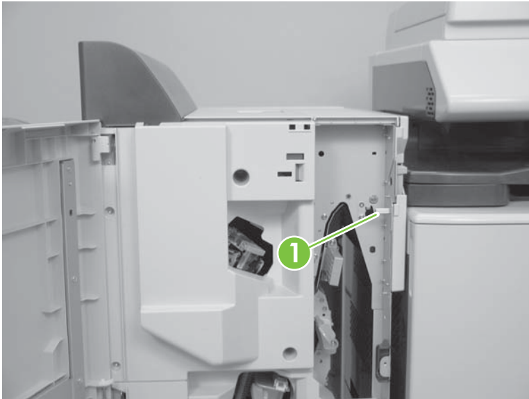
Figure 8-132 Remove output accessory (2 of 5)
