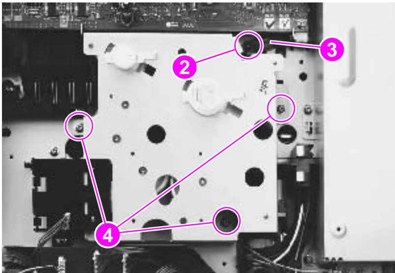
Figure 89. Feed-drive assembly
