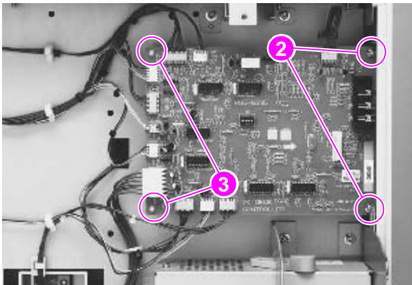
Figure 111. Controller board (2 of 2)
