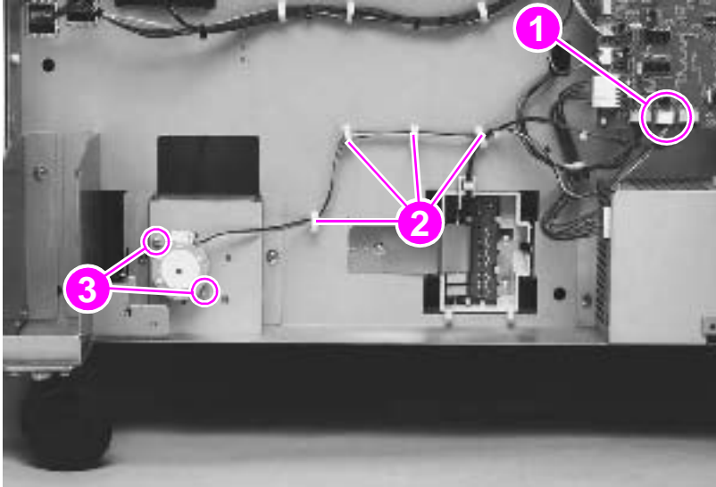
Figure 108. Drive motor
