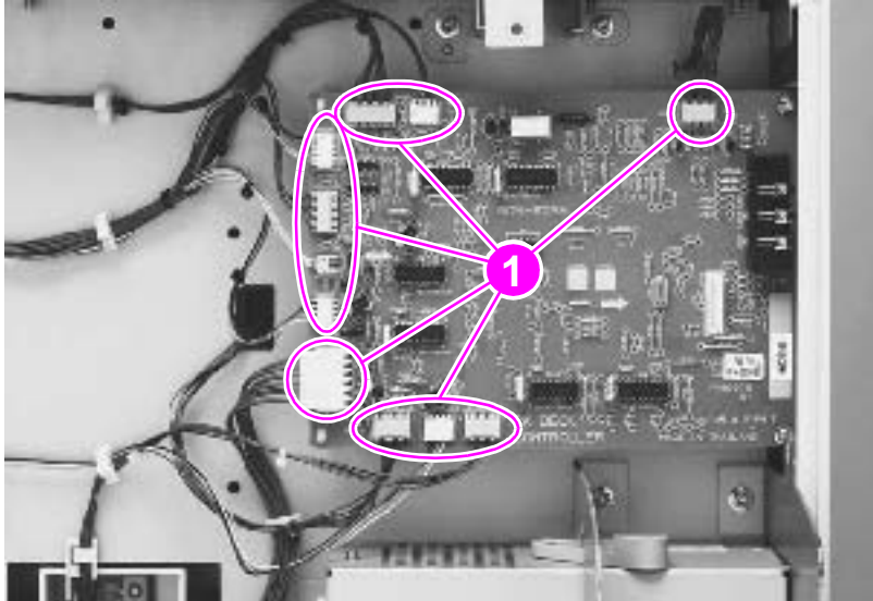
Figure 110. Controller board (1 of 2)
