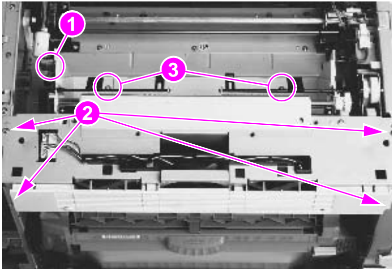
Delivery assembly
