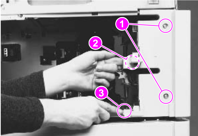
Figure 48. Rail covers
