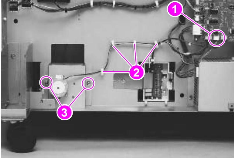
Figure 109. Drive assembly
