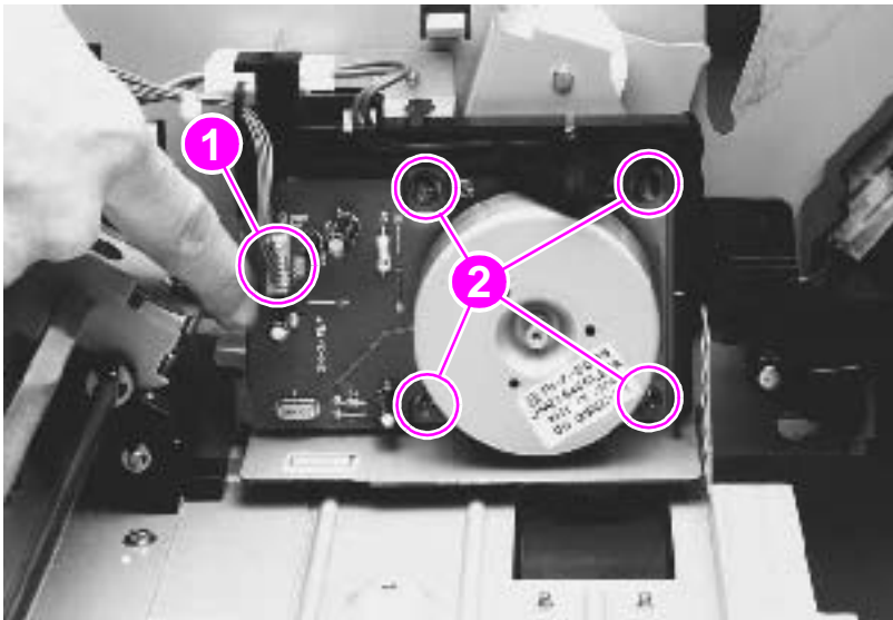
Figure 55. Delivery motor
